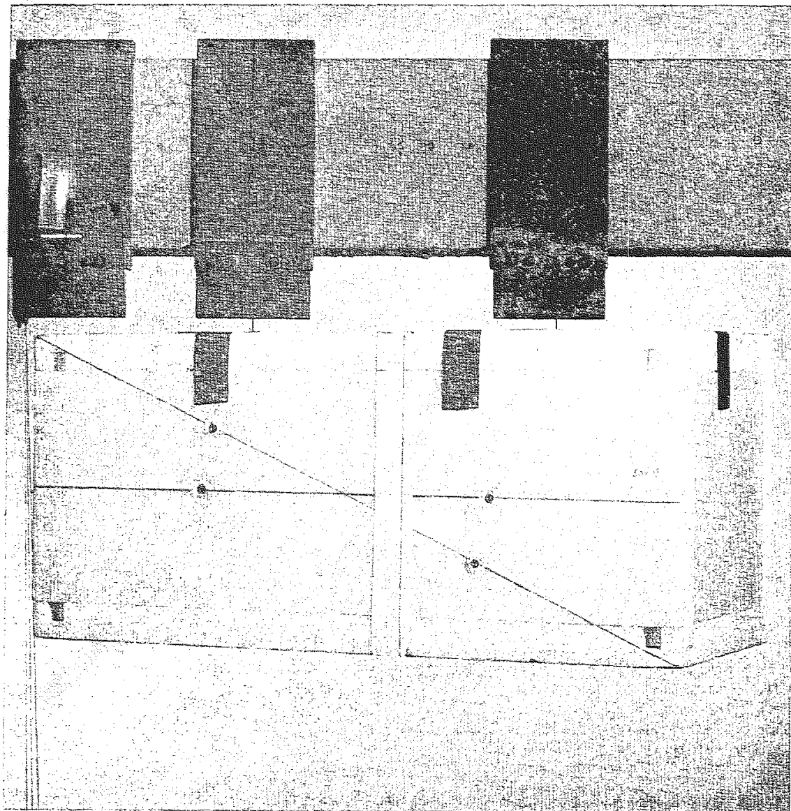
FIGURE 21. SPECIMEN HOLDER IN PLACE FOR MOMENT OF INERTIA MEASUREMENT (YZ AXES).
