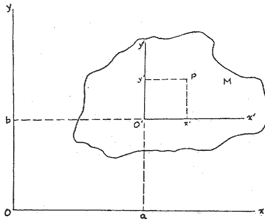
FIGURE 4. AXIS SYSTEM FOR PARALLEL AXIS TRANSFORMATION.
