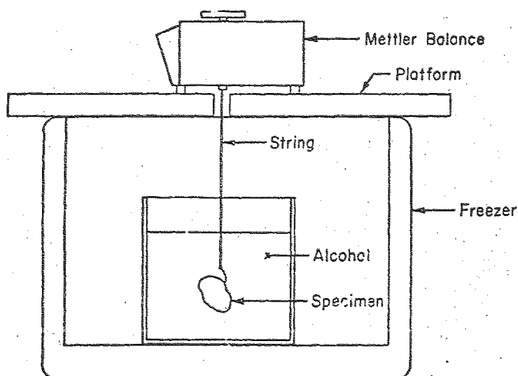
FIGURE 23. SCHEMATIC OF UNDER ALCOHOL WEIGHING DEVICE.
